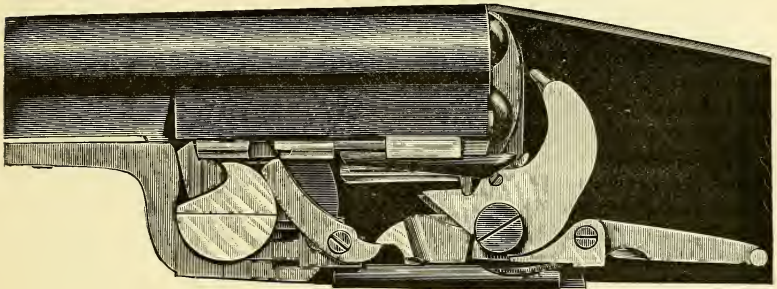
W. W. Greener's "Unique" Hammerless Ejector.
